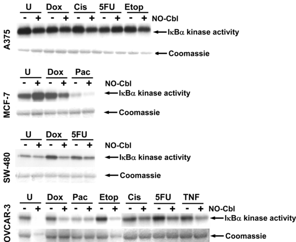
Figure 3. \text{I}\kappa\text{B} kinase (IKK) activity. IKK activity was assessed using recombinant GST- \text{I}\kappa\text{B}\alpha(1-54) and \gamma^{32}\text{P} -ATP as substrates. The phosphorylated GST fusion protein was detected by autoradiography. IKK activity was determined in cells that were pre-treated with NO-Cbl (300 \mu\text{M} , 16 h) followed by doxorubicin (20 \mu\text{M} , 4 h) or cisplatin (20 \mu\text{M} , 1 h) or 5 fluorouracil (5-FU, 100 \mu\text{M} , 5 h) or etoposide (20 \mu\text{M} , 4 h) or paclitaxel (20 \mu\text{M} , 5 h). Anti- \beta -actin antibody was used as an irrelevant antibody control for immunoprecipitation and yielded no signal. After exposure to film, the gel was stained with Coomassie blue to visualize total protein and demonstrated equal loading of the GST- \text{I}\kappa\text{B}\alpha(1-54) substrate. The same cell extracts were probed for total IKK by immunoblot analysis and demonstrated equal loading of IKK. doi:10.1371/journal.pone.0001313.g003
